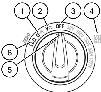
Figure 2: Rotary switch
