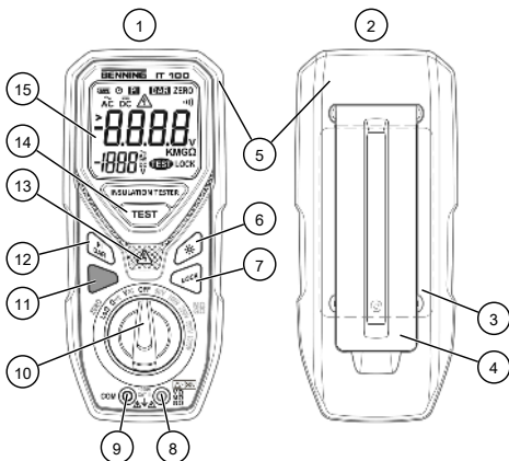
Figure 1: BENNING IT 100 device structure
